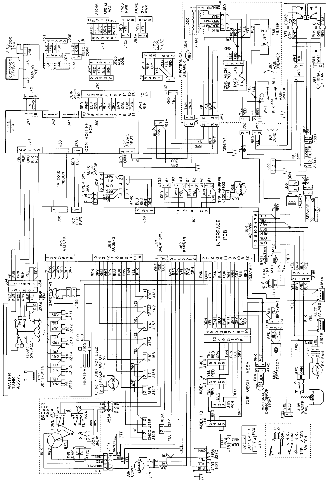
Figure 71. Wiring Diagram - 115 V
