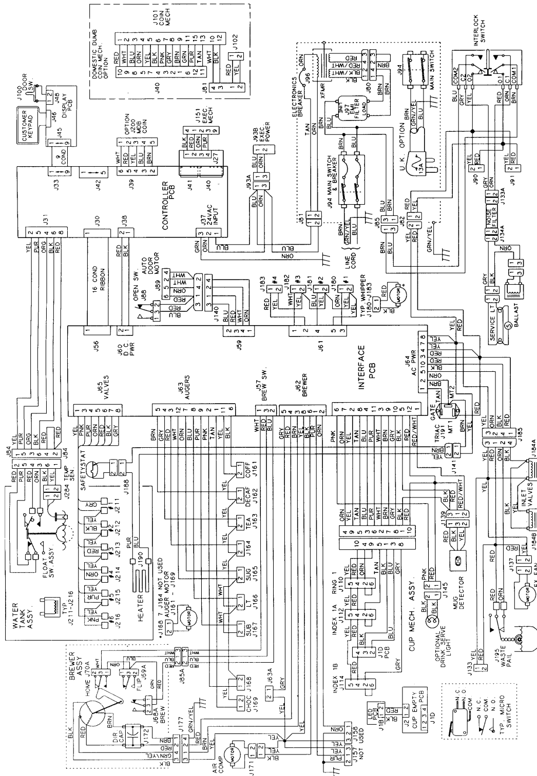
Figure 72. Wiring Diagram - 230 V
