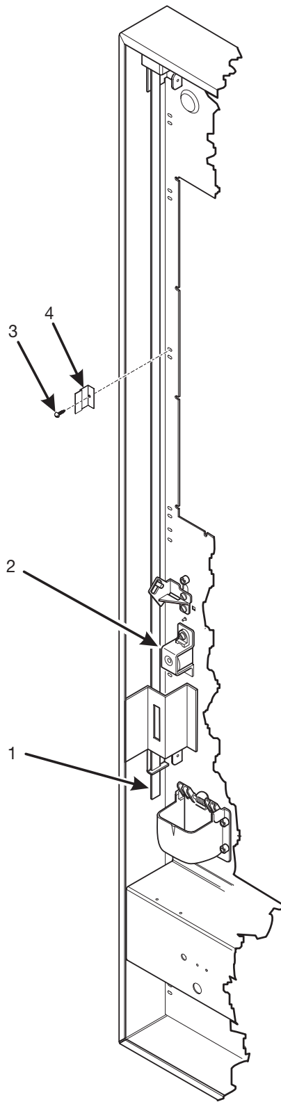
Figure 9. Door Lock Mechanism
